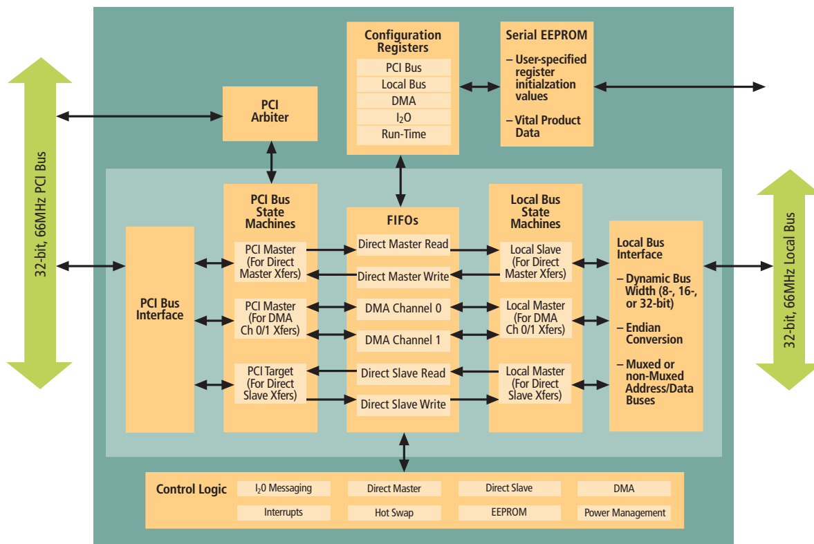
PCI 9056 Internal Block Diagram
