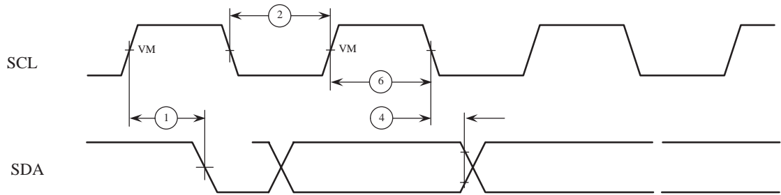
Figure 15: I²C Timing Diagram I
