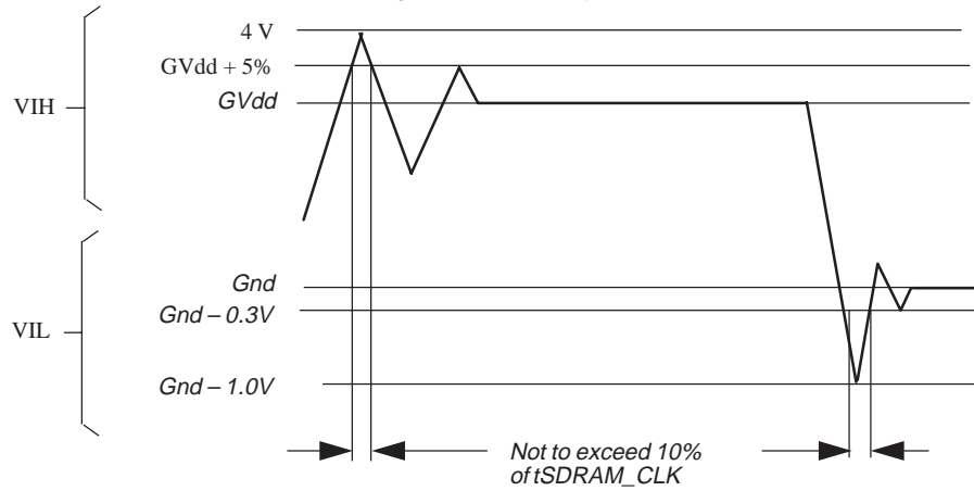
Figure 3: Overshoot/Undershoot Voltage
