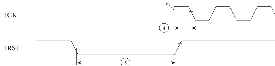
Figure 22: JTAG TRST Timing Diagram
