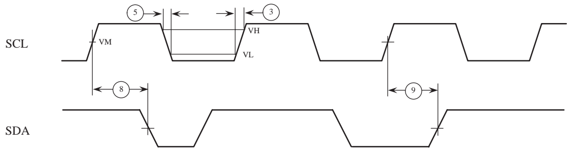
Figure 16: I²C Timing Diagram II
