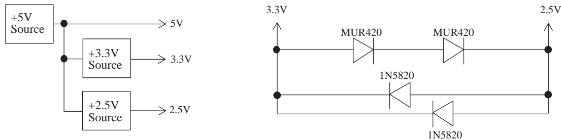
Figure 27: Example Voltage Sequencing Circuits
