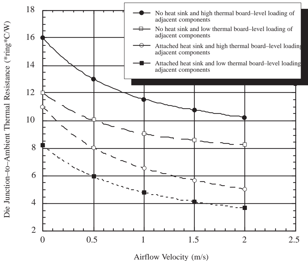
Figure 5: Die Junction-to-Ambient Resistance
