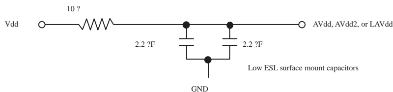
Figure 26: PLL Power Supply Filter Circuit
