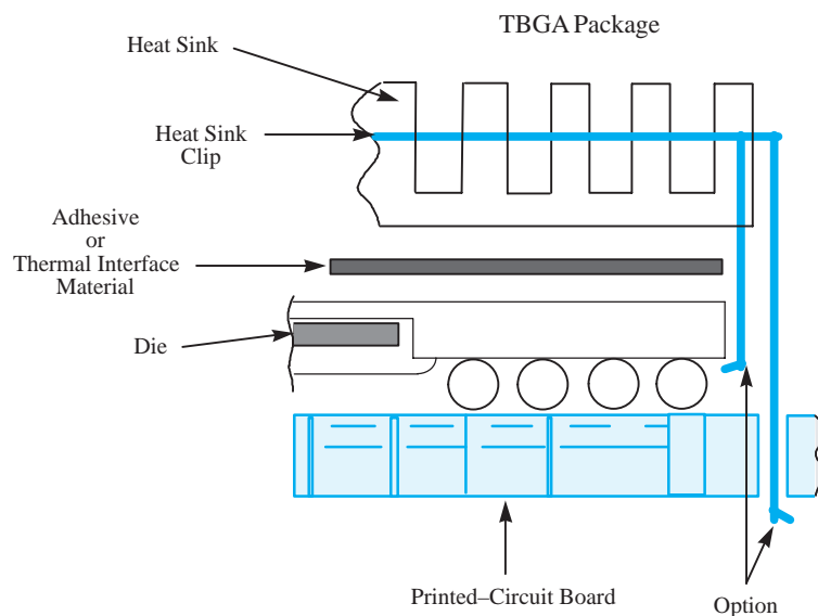
Figure 4: Package Exploded Cross-Sectional View with Several Heat Sink Options
