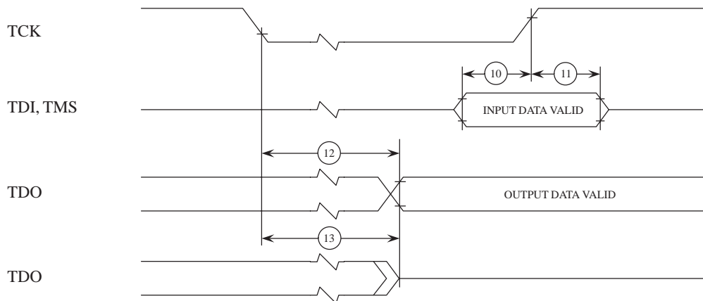
Figure 24: Test Access Port Timing Diagram
