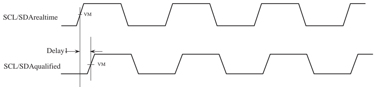
Figure 17: I²C Timing Diagram III
