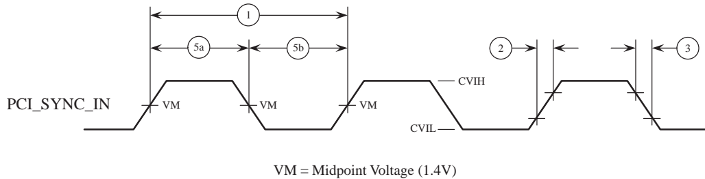
Figure 8: PCI_SYNC_IN Input Clock Timing Diagram
