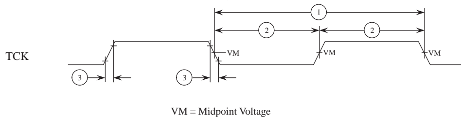
Figure 21: JTAG Clock Input Timing Diagram
