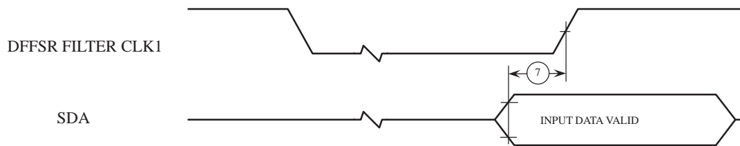
Figure 16: I²C Timing Diagram II
