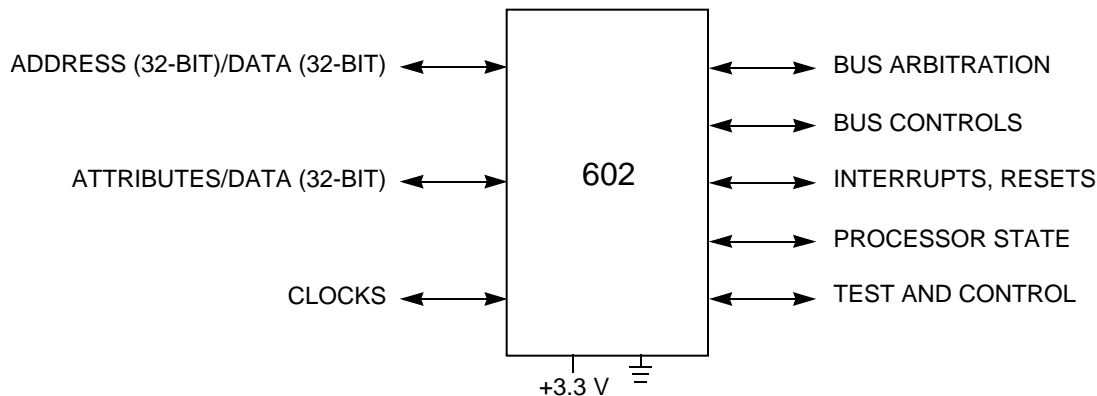
Figure 5. System Interface
