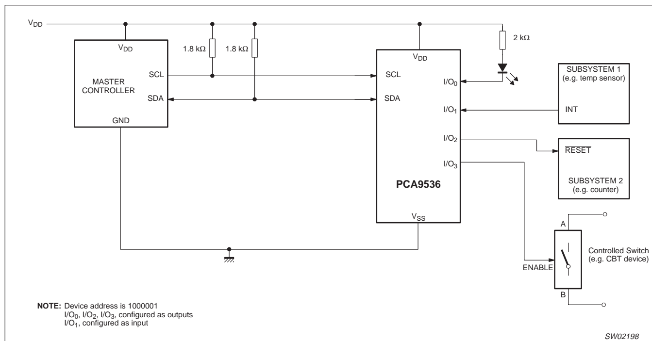
Figure 9. Typical application
