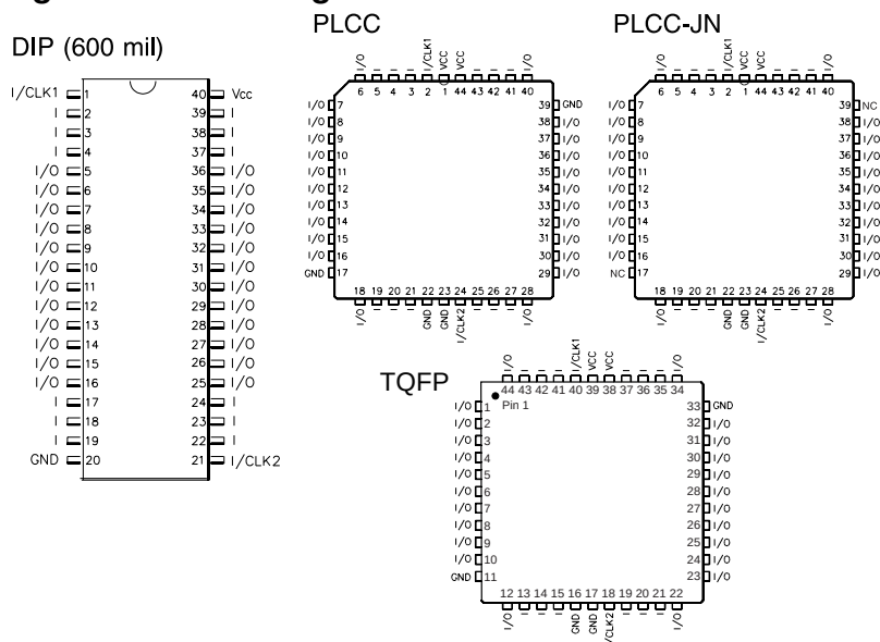
Figure 1: Pin Configuration
