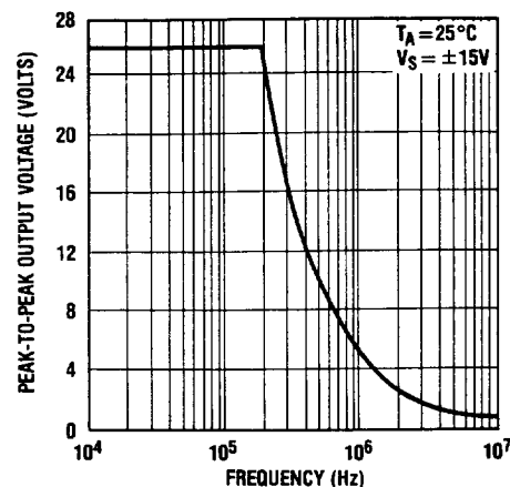
OP-37 Maximum Undistorted Output vs Frequency
