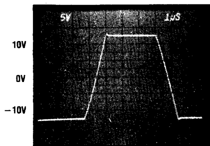
OP-37 Large Signal Response
