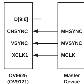
Figure 7 Slave Mode Connection
