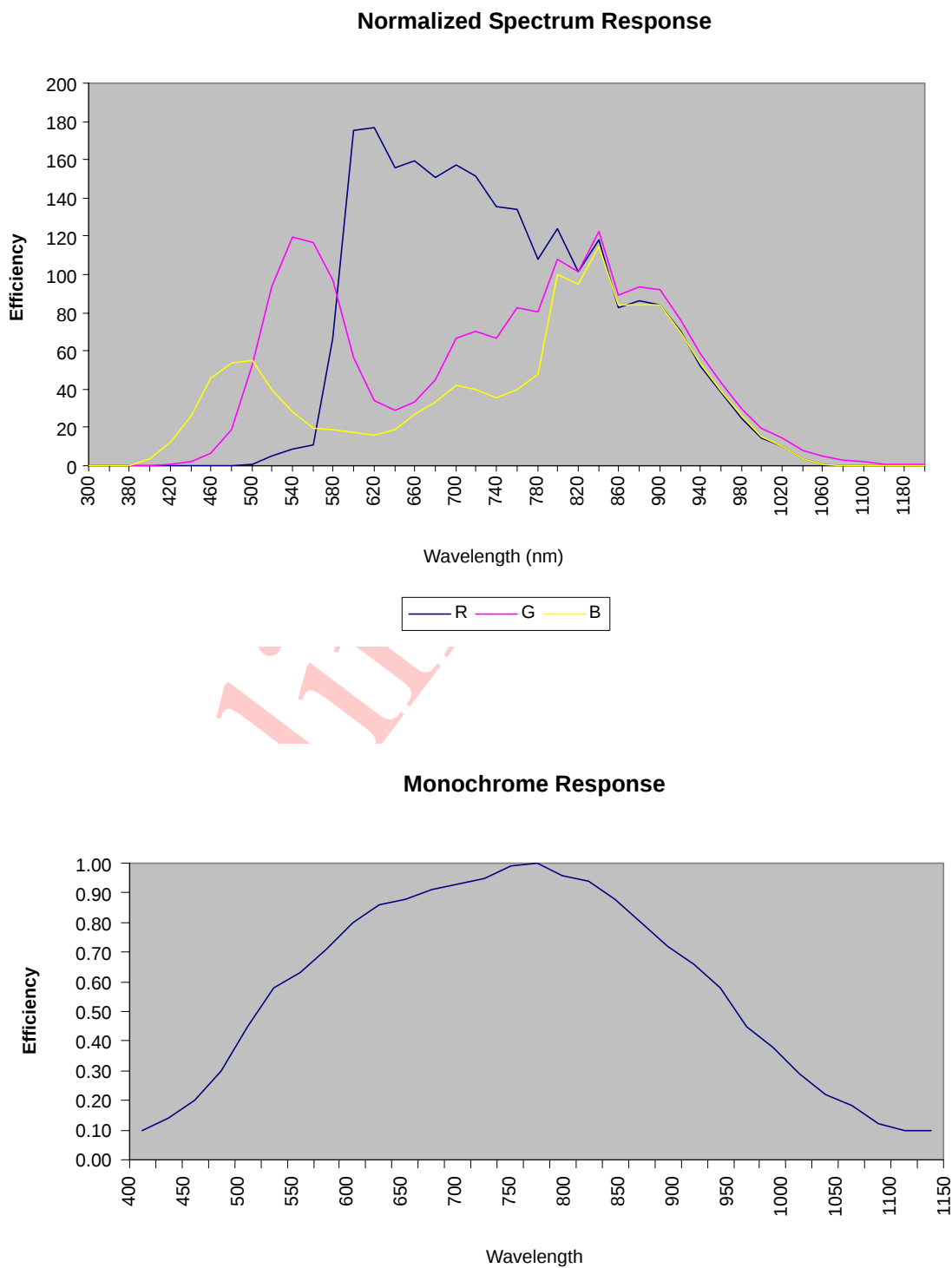
Figure 20 OV9625/OV9121 Light Response
