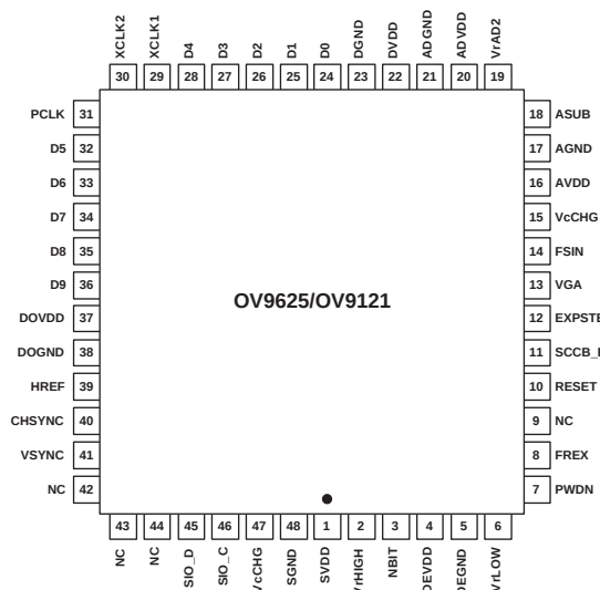
Figure 1 OV9625/OV9121 Pin Diagram
