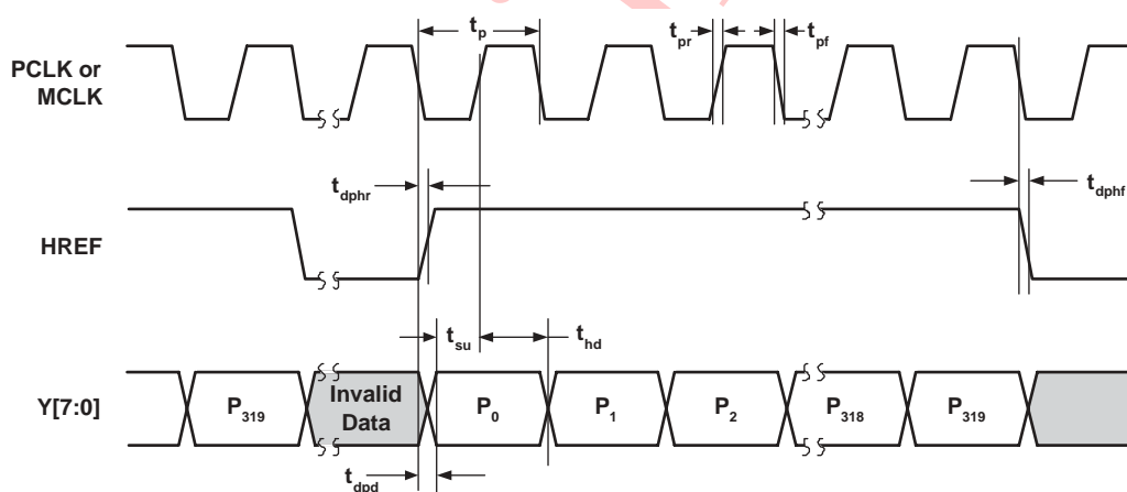
Figure 12 QVGA Line/Pixel Output Timing
