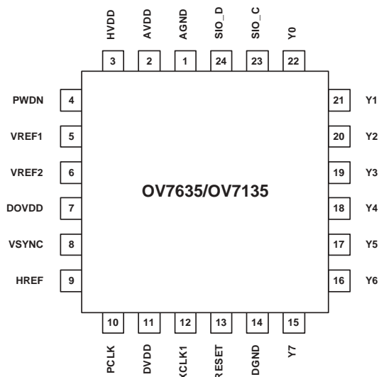
Figure 1 OV7635/OV7135 Pin Diagram
