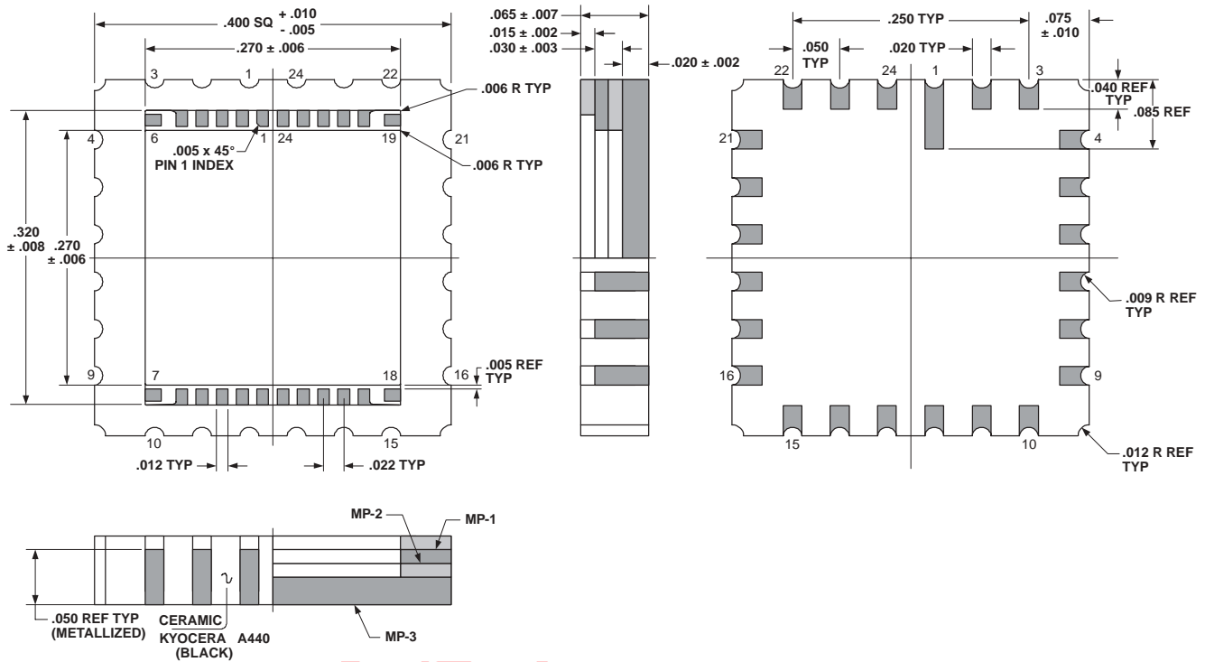
Figure 20 OV7635/OV7135 Package Specifications
