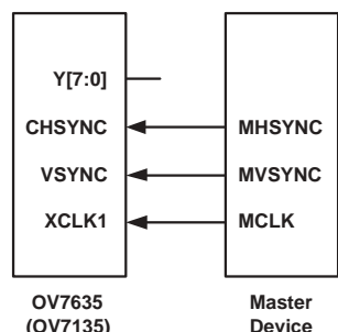
Figure 7 Slave Mode Connection
