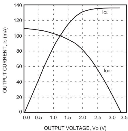
Figure 61. Slewlim ( T_J = 25^\circ\text{C} , V_{DD} = 3.3\text{ V} )
