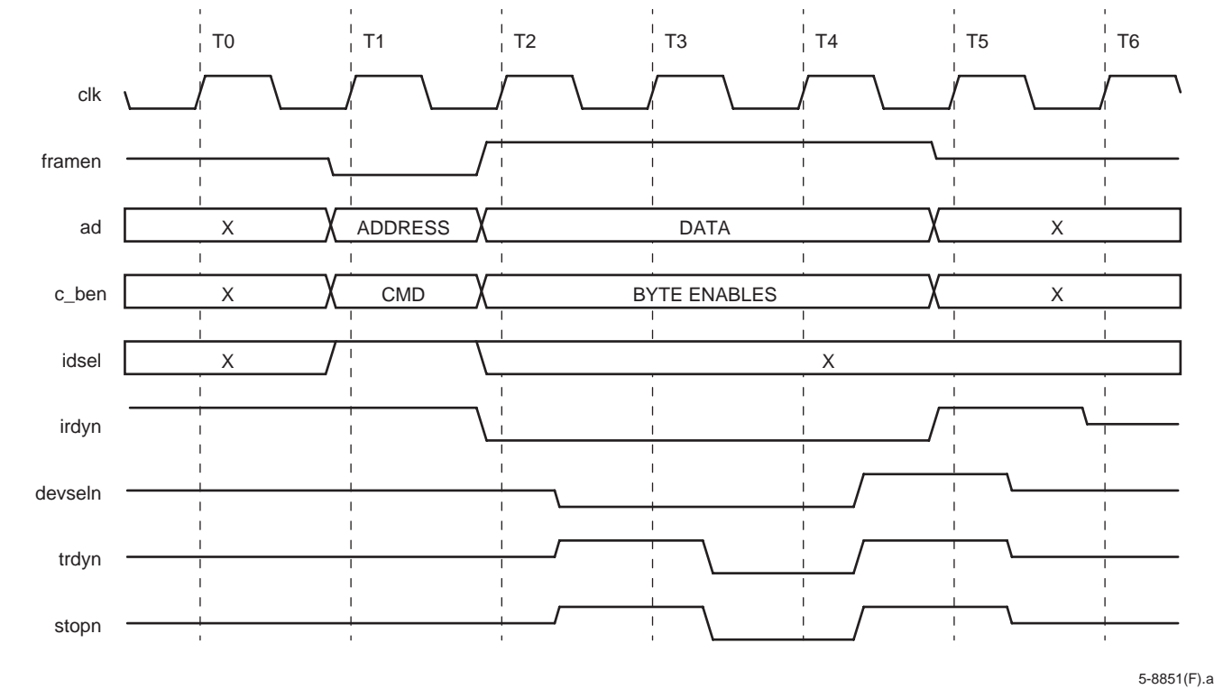
Figure 33. Target Configuration Write (PCI Bus, 64-Bit)
