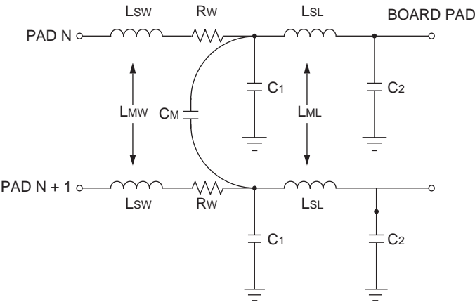
Figure 66. Package Parasitics
