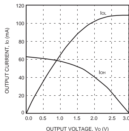
Figure 65. Fast ( T_J = 125^\circ\text{C} , V_{DD} = 3.0\text{ V} )
