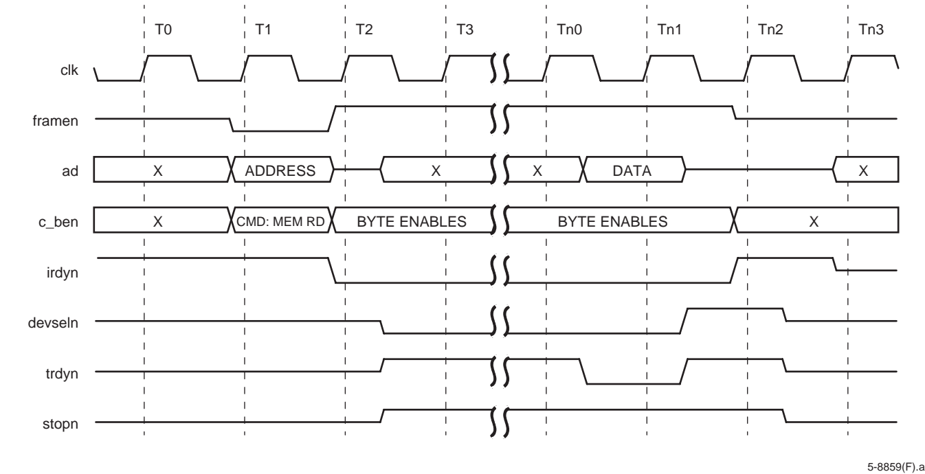
Figure 44. Target Memory Read Single, Not Delayed (PCI Bus, 64-Bit)
