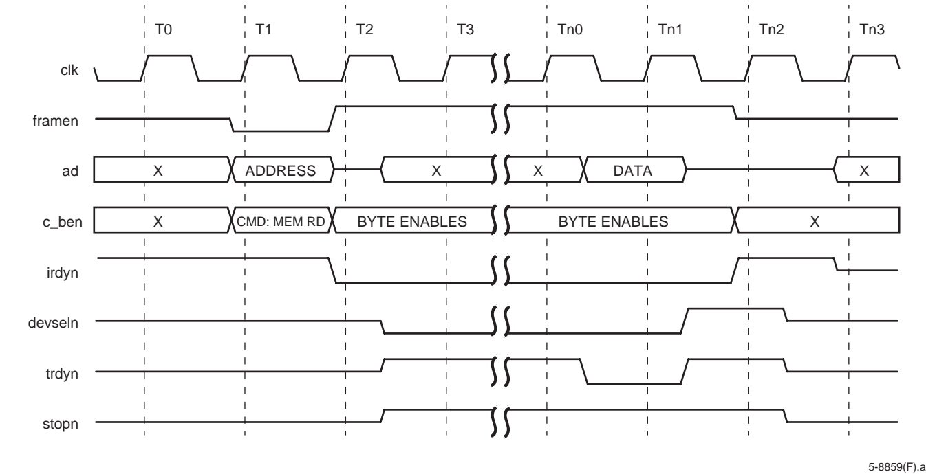
Figure 21. Target Memory Read Single, Not Delayed (PCI Bus, 64-Bit)
