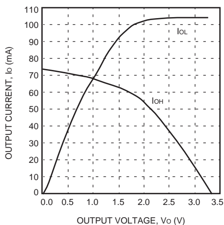
Figure 60. Sinklim ( T_J = 25^\circ\text{C} , V_{DD} = 3.3\text{ V} )
