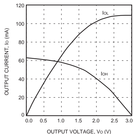
Figure 64. Slewlim ( T_J = 125^\circ\text{C} , V_{DD} = 3.0\text{ V} )
