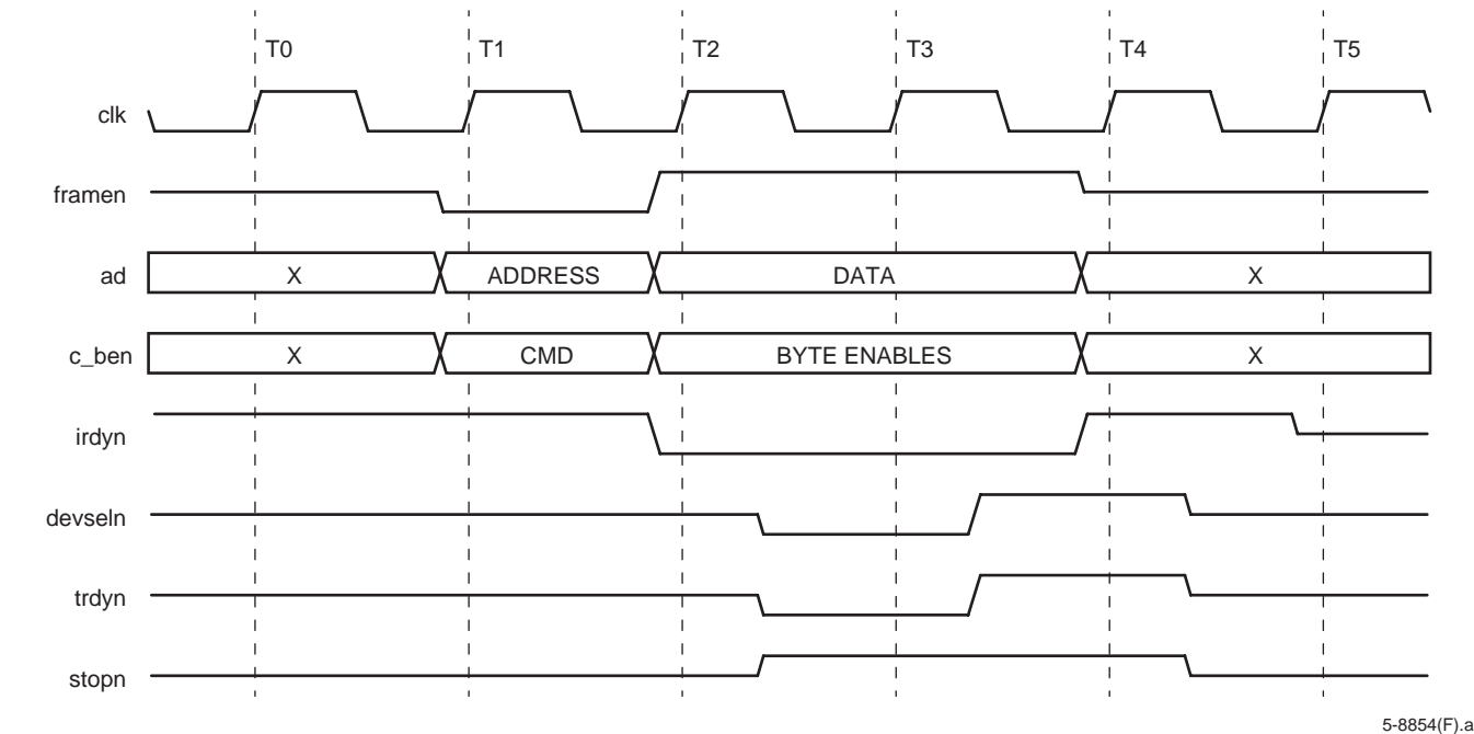
Figure 12. Target Write Memory Single (PCI Bus, 64-Bit)
