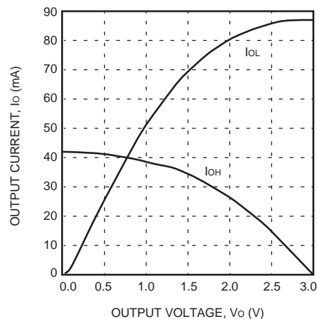
Figure 63. Sinklim ( T_J = 125^\circ\text{C} , V_{DD} = 3.0\text{ V} )
