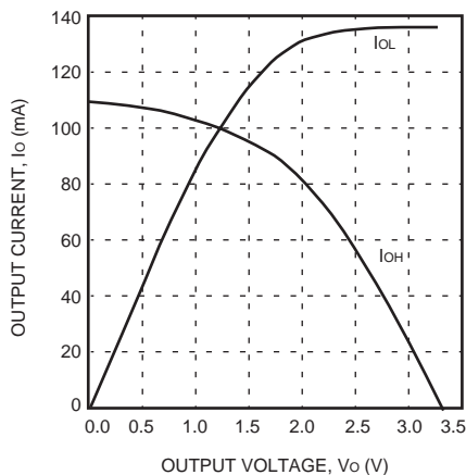
Figure 62. Fast ( T_J = 25^\circ\text{C} , V_{DD} = 3.3\text{ V} )
