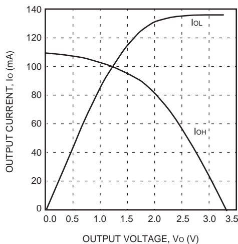
Figure 27. Fast ( T_J = 25^\circ\text{C} , V_{DD} = 3.3\text{ V} )
