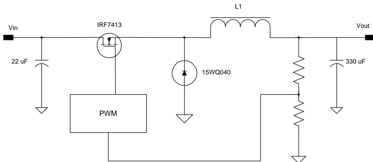
Simplified Schematic
