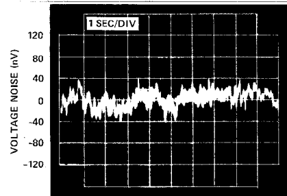
0.1Hz TO 10Hz PEAK-TO-PEAK NOISE
