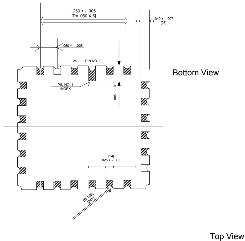
Figure 8. OV7635/OV7135 Package Diagram
