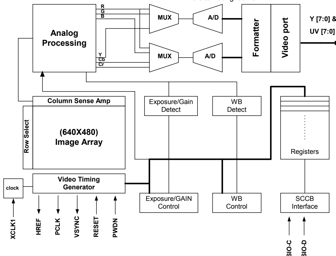
Figure 3. OV7635/OV7135 CMOS Image Sensor Block Diagram
