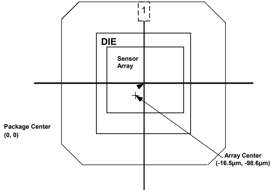
Figure 8. OV7635/7135 Sensor array center location
