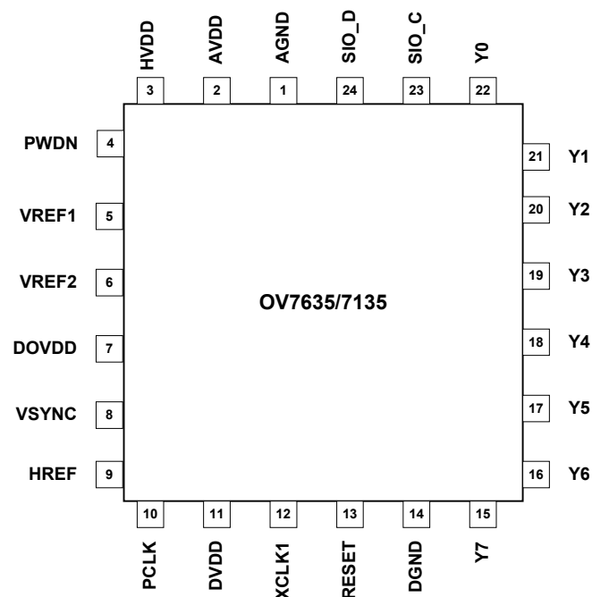
Figure 1. OV7635/OV7135 Pin Diagram
