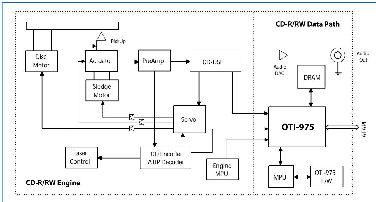
Block Diagram of CD-Recordable/ReWritable Drive Electronics
