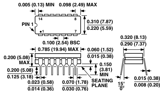
14-Lead Cerdip (Y Suffix) (Q-14)
