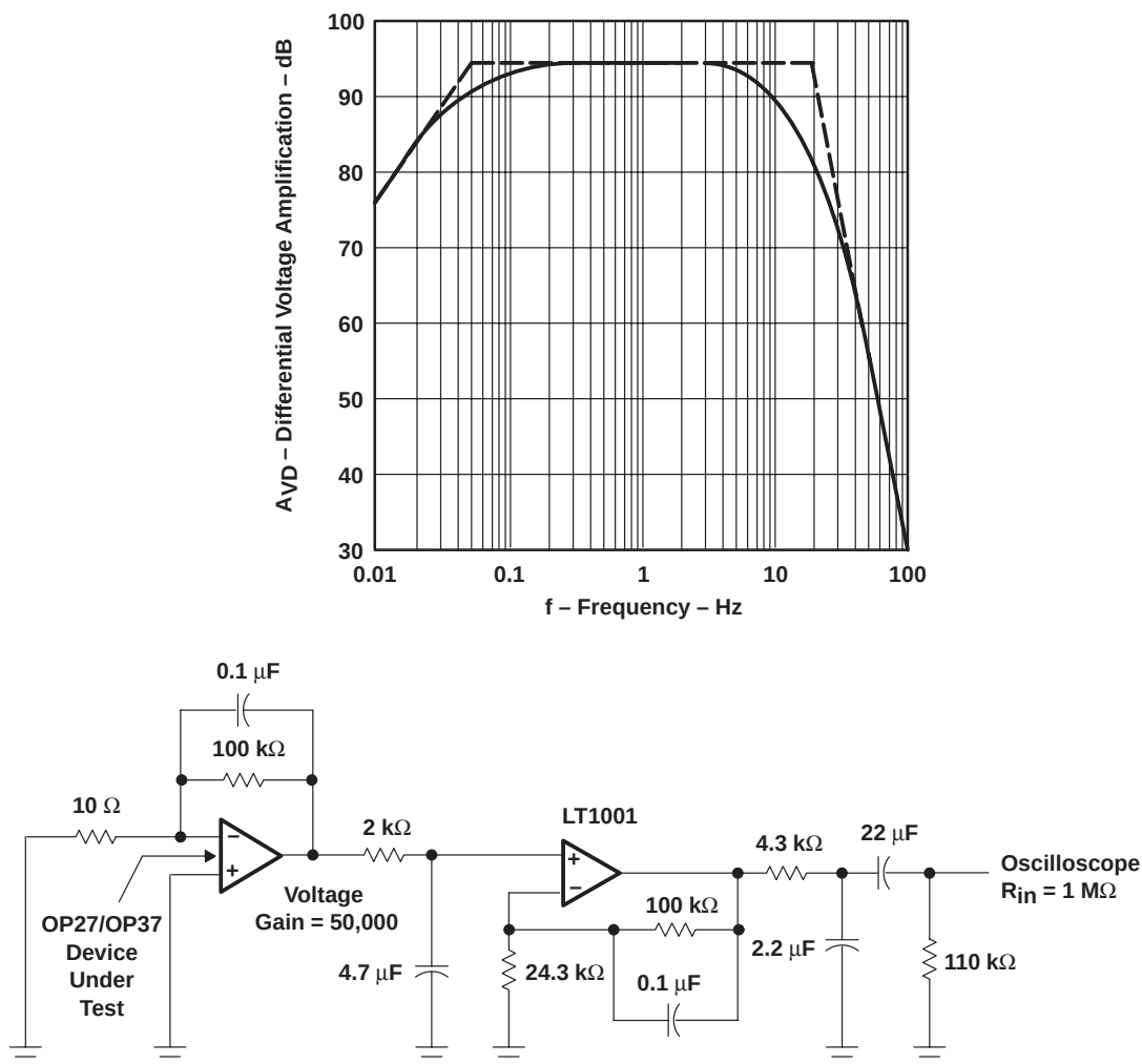
Figure 34. 0.1-Hz to 10-Hz Peak-to-Peak Noise Test Circuit and Frequency Response
