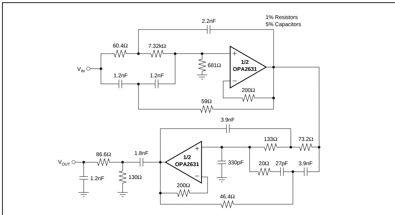
FIGURE 3. Bandpass Filter.
