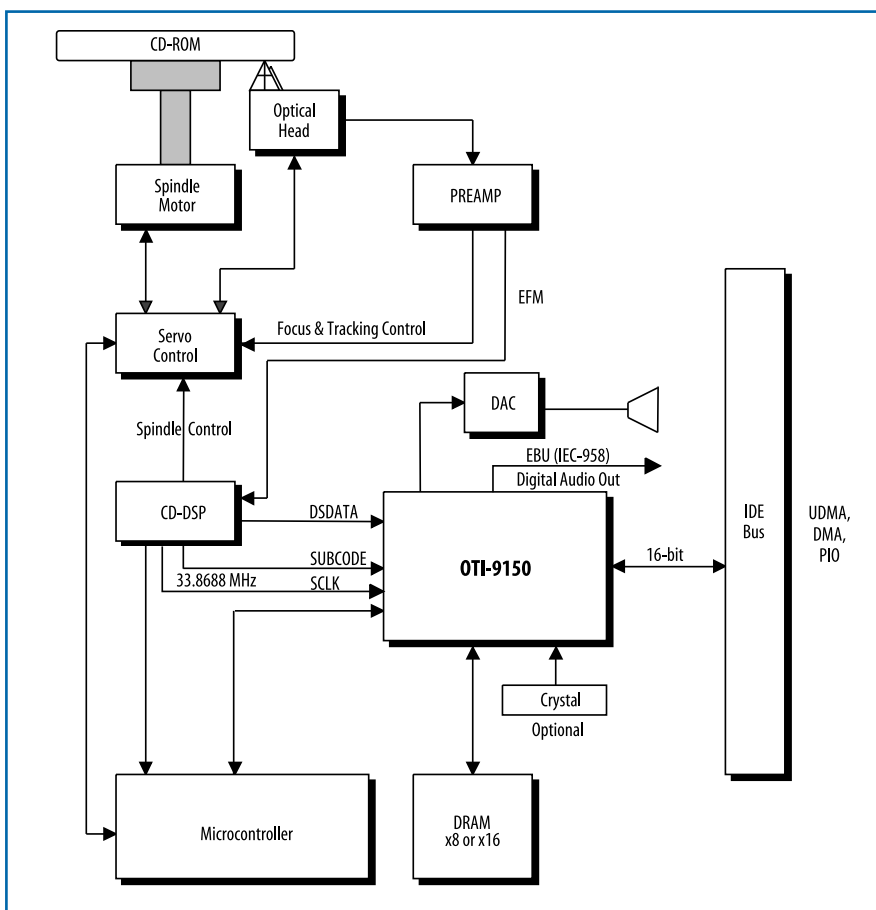
Block Diagram of CD-ROM Drive Electronics
