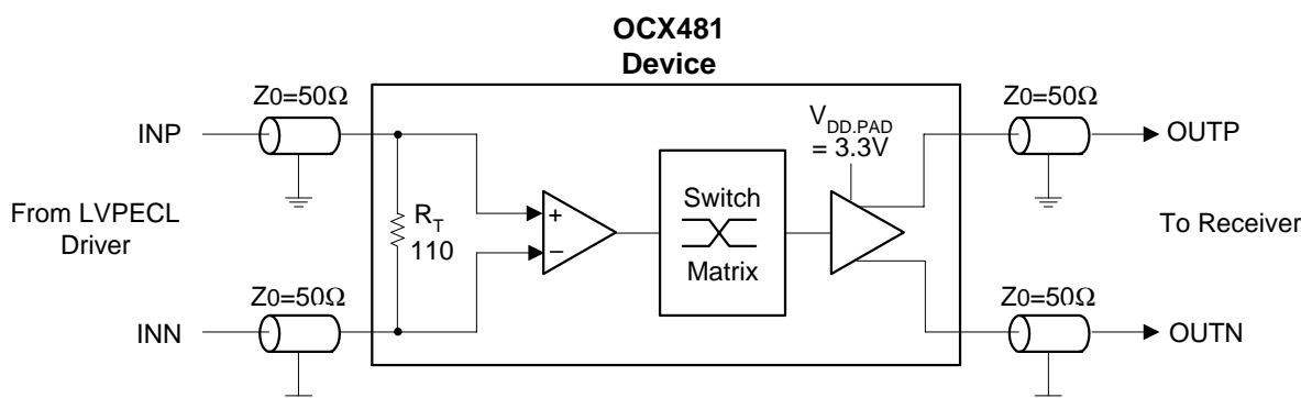
Figure 4 OCX481 Operating in LVPECL Mode
