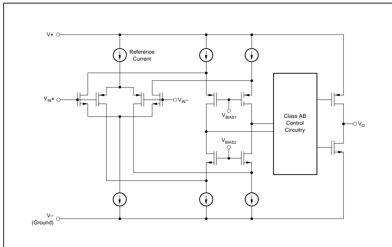
FIGURE 1. Simplified Schematic.
