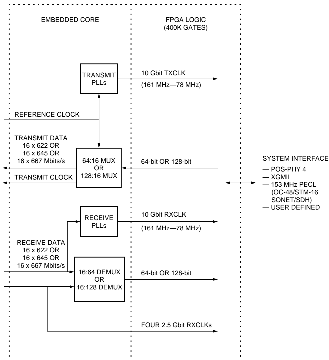
Figure 1. ORLI10G Block Diagram
