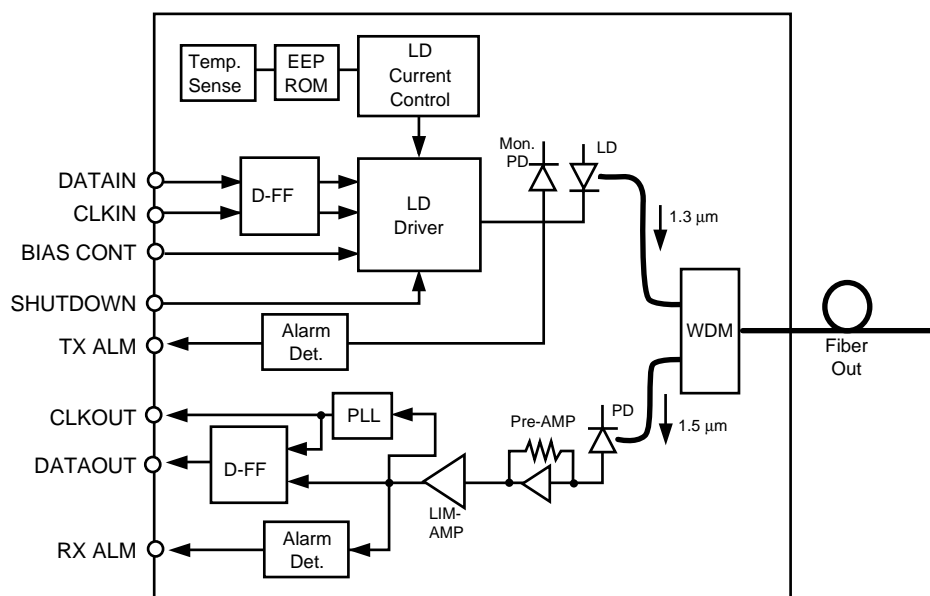
Figure 1. Block diagram of OD-B6212-ONUB.
