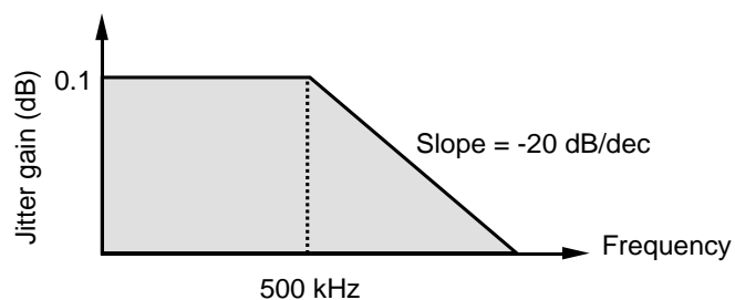
FIGURE 3. Jitter transfer mask
