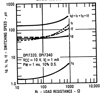
Switching Speed vs Load Resistance
