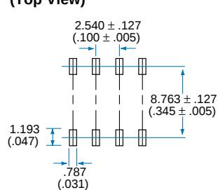
PC Board Pattern (Top View)
