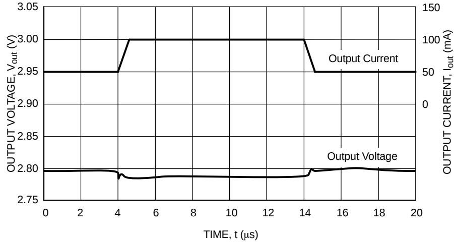
Figure 29. (continued) Load Transient Response ( t_r = t_f = 0.5 \mu\text{s} , C_{in} = 1.0 \mu\text{F} )
