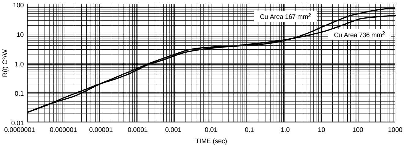
Figure 7. Single-Pulse Heating Curves, D²PAK 5-Lead
