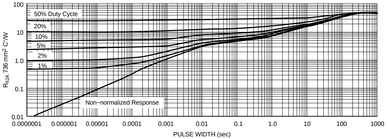
Figure 8. Duty Cycle for 1" Spreaders Boards, DPAK 5-Lead
