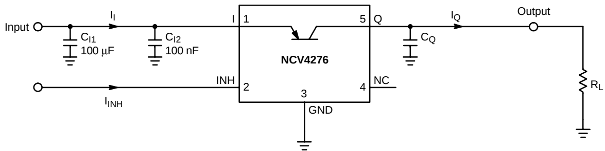
Figure 2. Measuring Circuit
