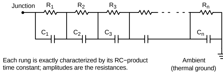
Figure 11. Non-Grounded Capacitor Thermal Ladder ("Foster" Ladder)
