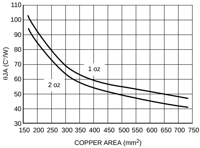
Figure 4. \theta_{JA} vs. Copper Spreader Area, DPAK 5-Lead
