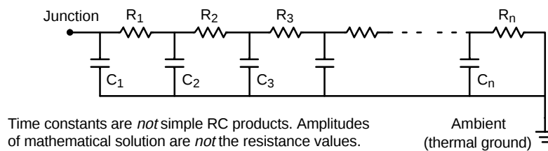
Figure 10. Grounded Capacitor Thermal Network ("Cauer" Ladder)
