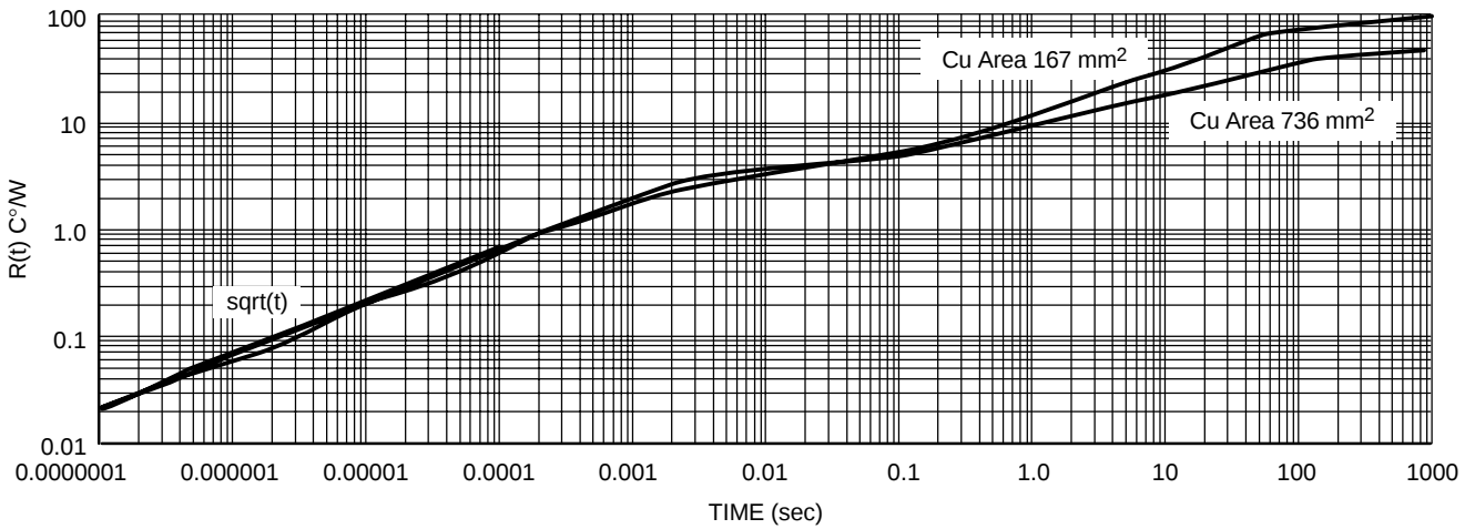
Figure 6. Single-Pulse Heating Curves, DPAK 5-Lead
