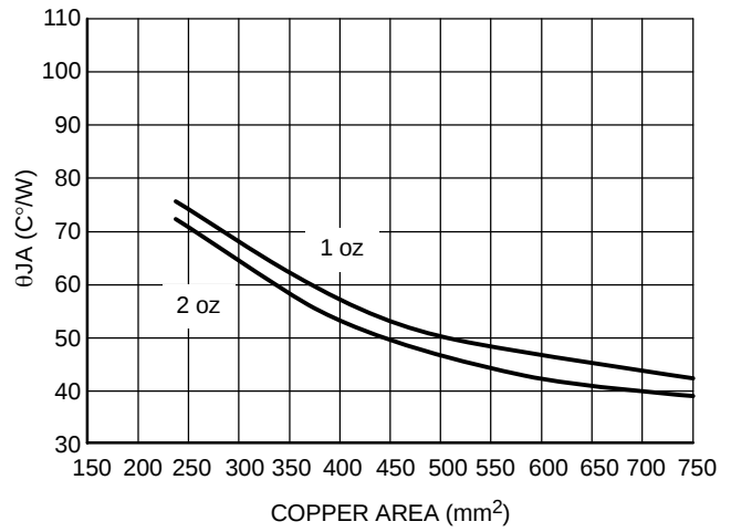
Figure 5. \theta_{JA} vs. Copper Spreader Area, D²PAK 5-Lead
