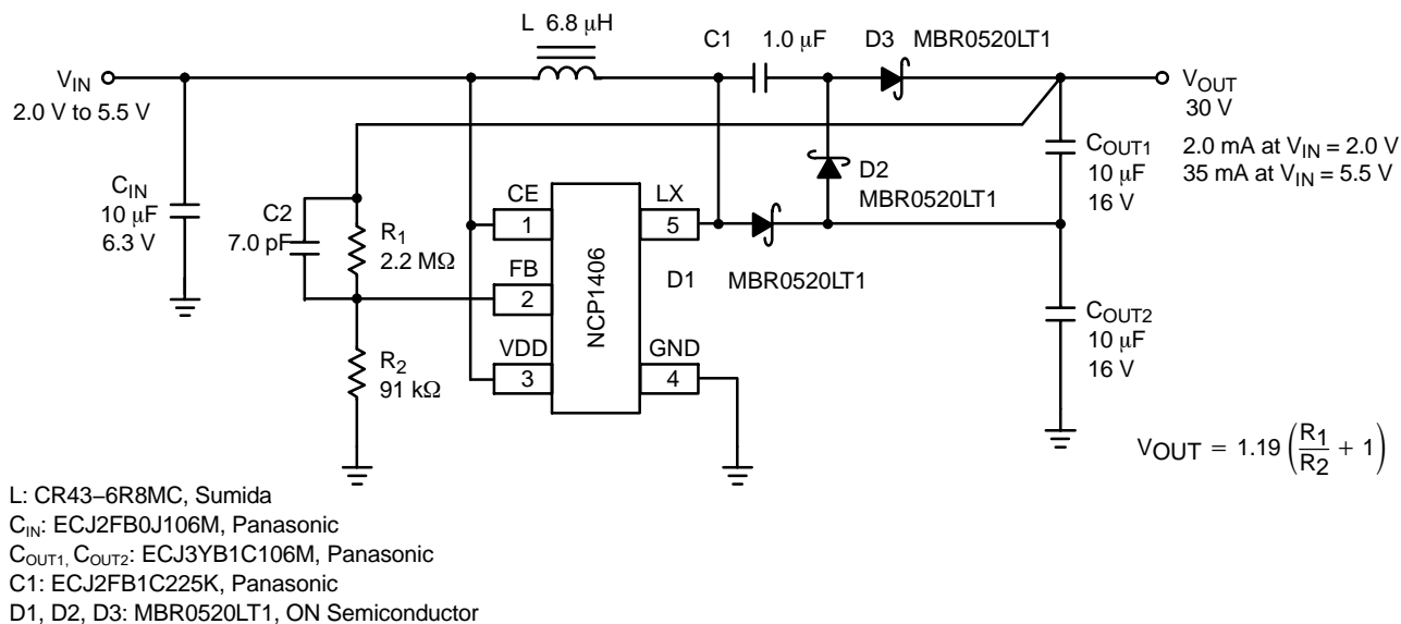
Figure 53. Step-Up DC-DC Converter with 30 V Output Voltage
