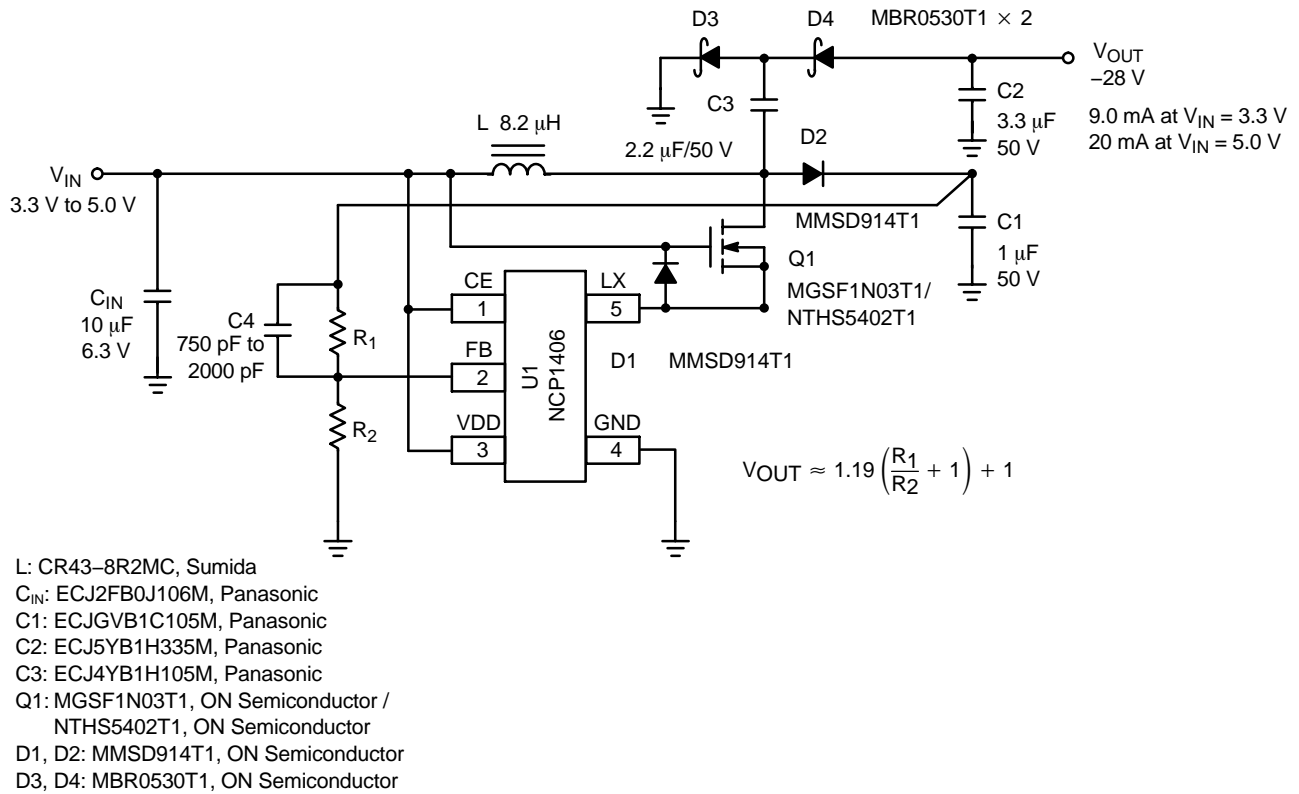
Figure 54. Voltage Inverting DC-DC Converter with -28 V Output Voltage
