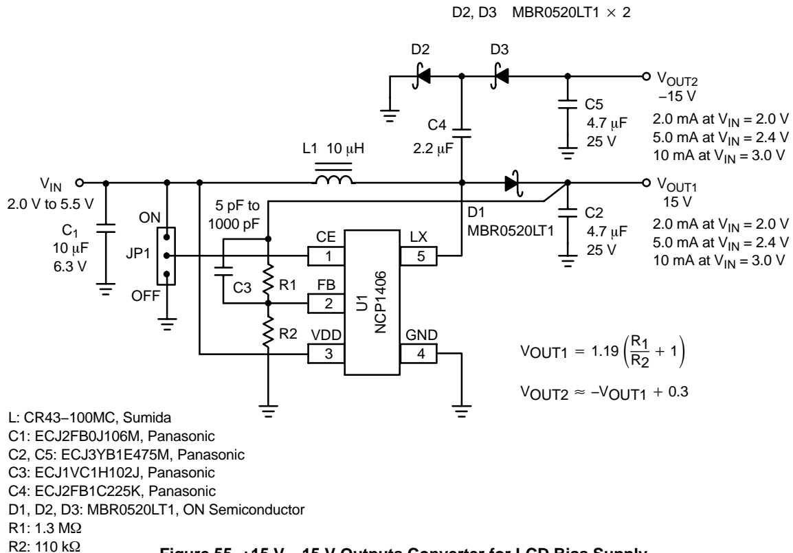
Figure 55. +15 V, -15 V Outputs Converter for LCD Bias Supply
