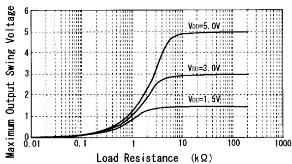
Maximum Output Swing Voltage vs. Load Resistance
