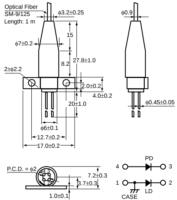
NDL7705P1
