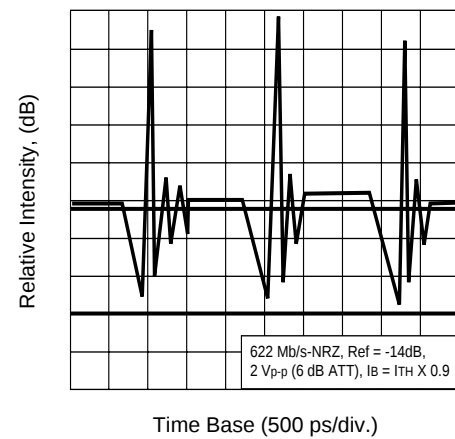
EYE DIAGRAM
