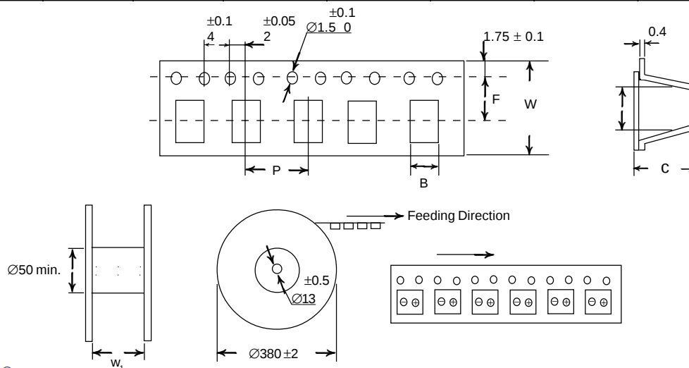
Case Size W+/-0.2 A+/-0.1 B+/-0.2 C+/-0.1 P+/-0.1 F+/-0.05 W1+/-0.5 Reel Qty. 3.8x3.8x6.5 12.0 7.0 4.1 4.1 8.0 5.5 13.5 3000 3.8x3.8x9.5 16.0 10.0 4.1 4.1 8.0 7.5 17.5 3000 4.8x4.8x7.3 16.0 7.7 5.0 5.2 8.0 7.5 17.5 2500 4.8x4.8x10.3 16.0 10.7 5.0 5.2 8.0 7.5 17.5 2500
