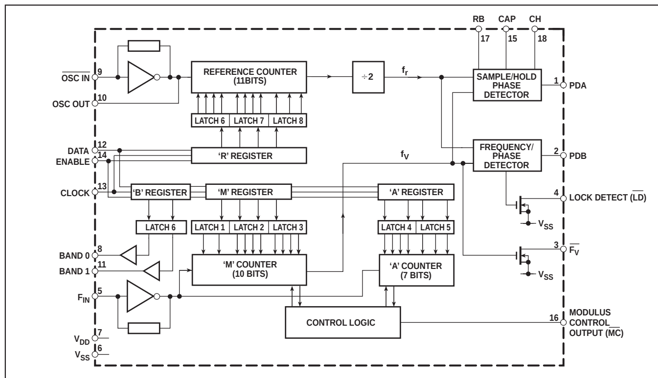
Fig.2 Block diagram
