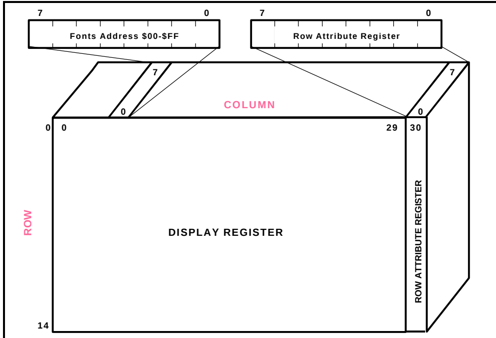
Figure 4. Memory Map of Display Register (Row 0 - 14)
