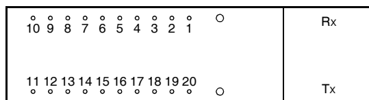
Figure 1. Top View of the NLT02-80-PA Transceiver, 20-Pin Configuration
