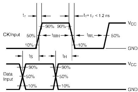
FIGURE 5. AC Waveforms
