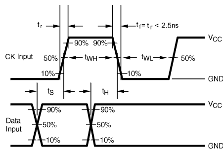
FIGURE 4. AC Waveforms
