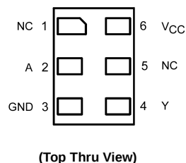
Pad Assignments for MicroPak
