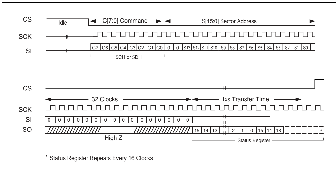
Figure 11. Transfer Sector to SRAM Command Sequence
