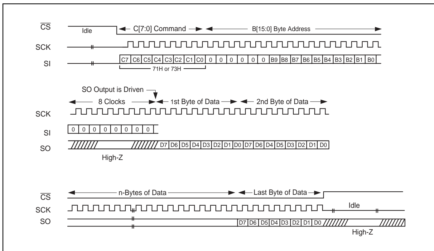
Figure 11. Read from SRAM Command Sequence
