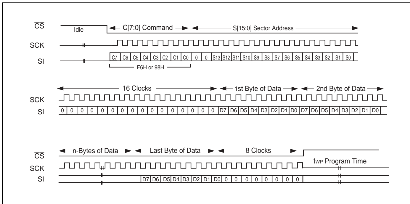
Figure 10. Write to Sector using SRAM Command Sequence
