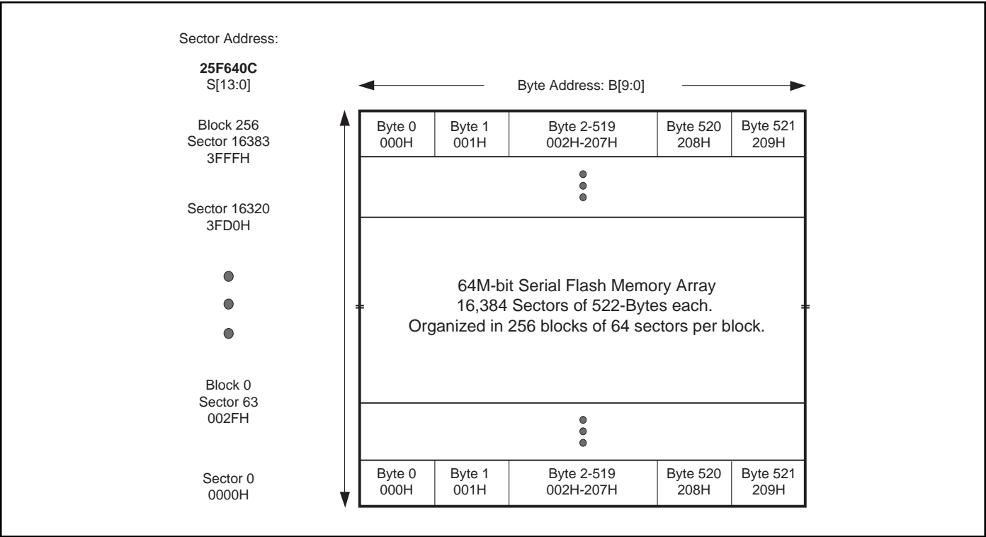
Figure 3. NX25F640C Serial Flash Memory Array
