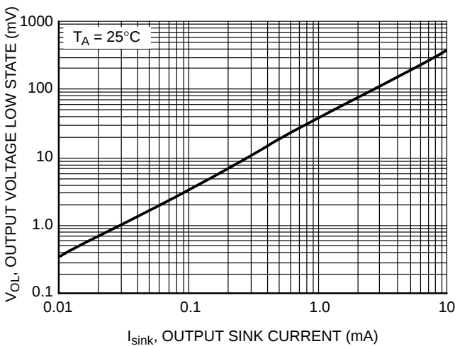
Figure 5. NCS2300 Series Output Voltage Low State vs. Output Sink Current
