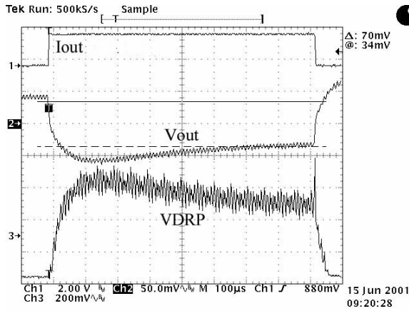
Figure 21. V_{DRP} Tuning Waveforms. The RC Time Constant of the Current Sense Network Is Too Short (Fast): V_{DRP} and V_{OUT} Both Overshoot.
