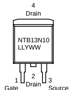
D 2 PAK CASE 418B STYLE 2
