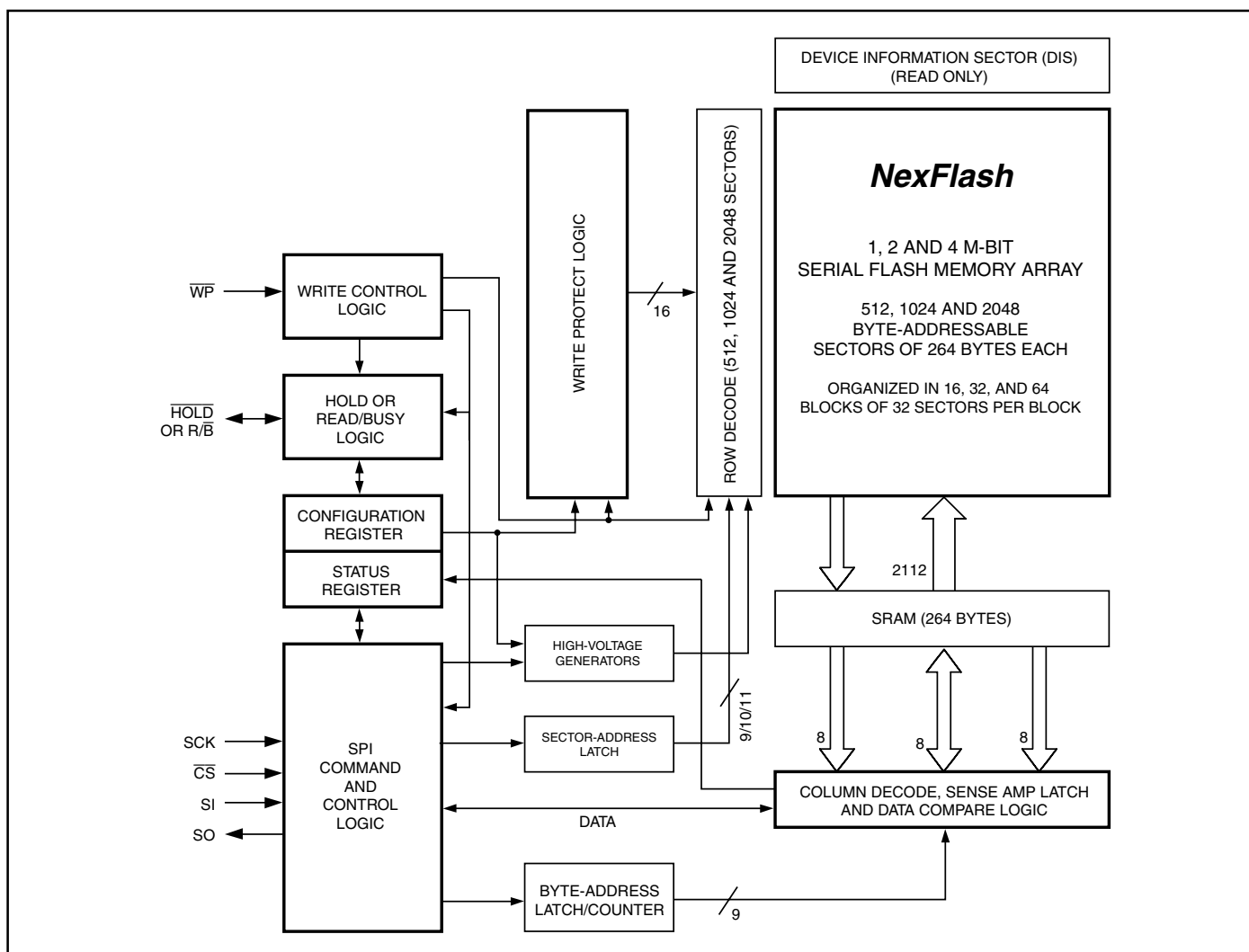
Figure 2. NX25F011B, NX25F021B, and NX25F041B Architectural Block Diagram
