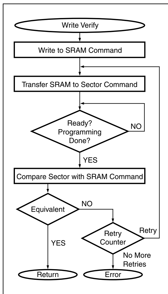
Figure 12. Write/Verify Flow
