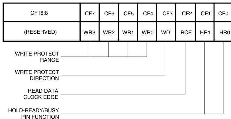
Figure 7. Configuration Register Bit Locations
