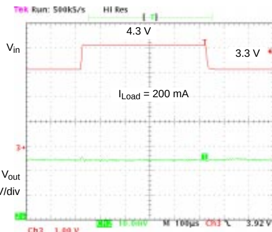
Figure 10. Line Transient
