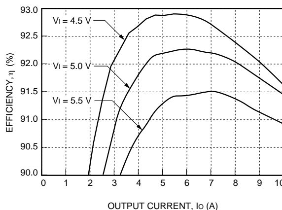
Figure 23. NH033F-L Efficiency, T_A = 25\text{ }^{\circ}\text{C}
