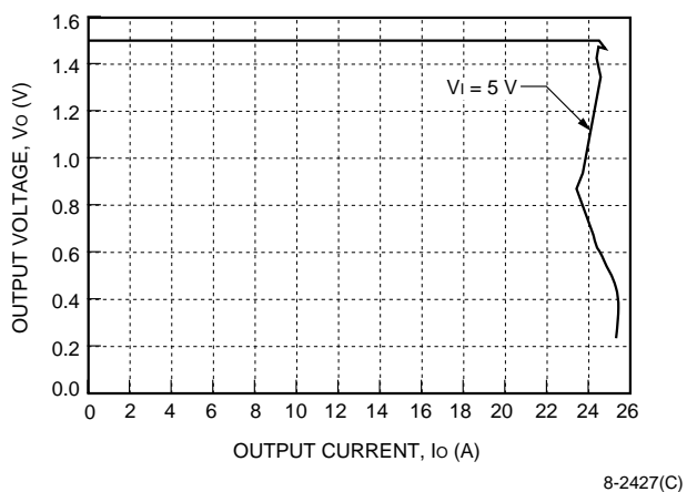
Figure 10. NH050M-L Current Limit, T_A = 25^\circ\text{C}
