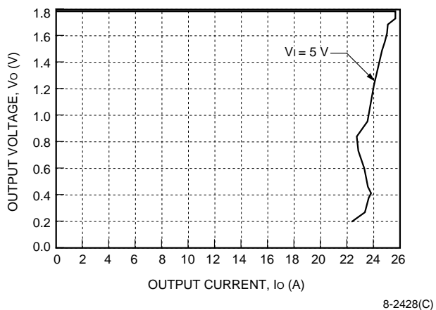
Figure 12. NH050S1R8-L Current Limit, T_A = 25^\circ\text{C}
