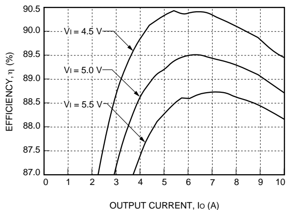
Figure 21. NH033G-L Efficiency, T_A = 25\text{ }^{\circ}\text{C}
