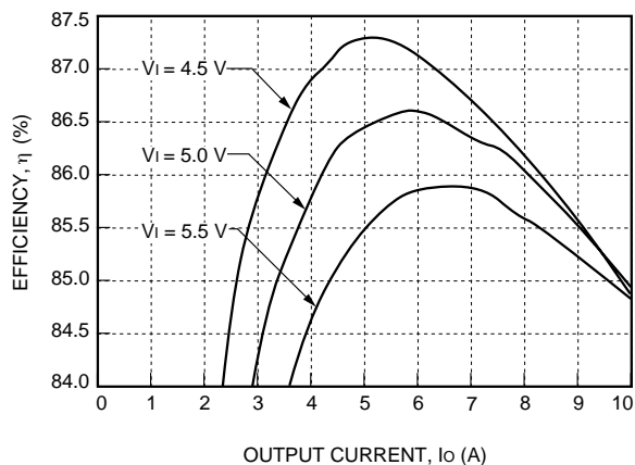
Figure 19. NH033S1R8-L Efficiency, T_A = 25\text{ }^{\circ}\text{C}
