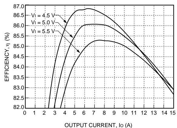
Figure 20. NH050S1R8-L Efficiency, T_A = 25\text{ }^{\circ}\text{C}
