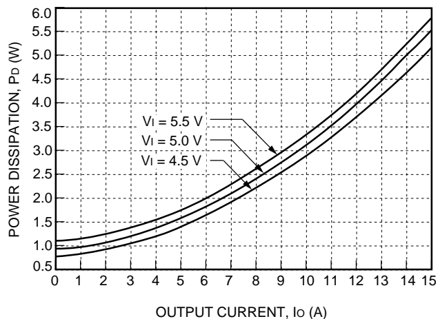
Figure 47. NH050G-L Typical Power Dissipation vs. Output Current, T_A = 25\text{ }^{\circ}\text{C}
