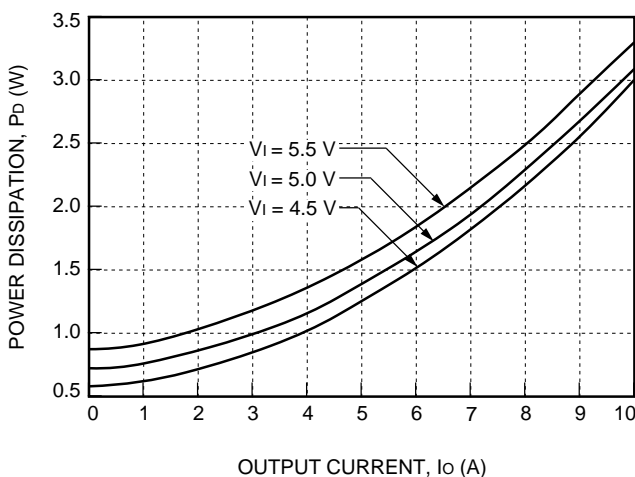
Figure 48. NH033F-L Typical Power Dissipation vs. Output Current, T_A = 25\text{ }^{\circ}\text{C}
