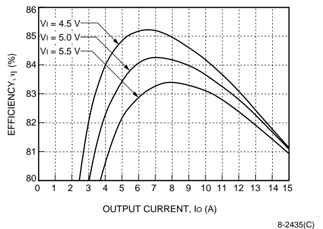
Figure 18. NH050M-L Efficiency, T_A = 25\text{ }^{\circ}\text{C}
