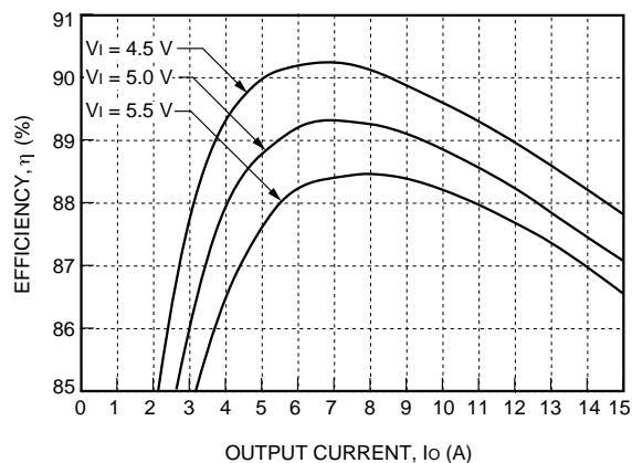
Figure 22. NH050G-L Efficiency, T_A = 25\text{ }^{\circ}\text{C}
