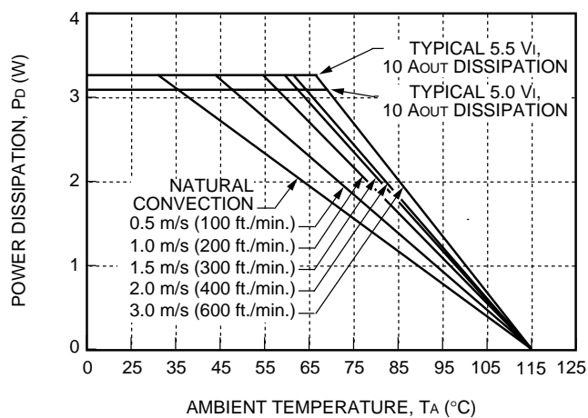
Figure 50. NH033x-L Power Derating vs. Local Ambient Temperature and Air Velocity
