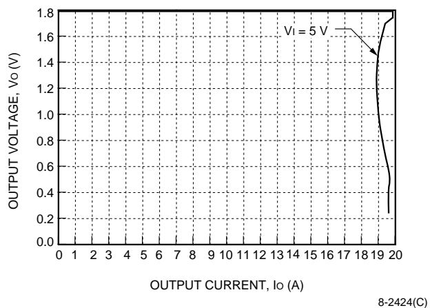
Figure 11. NH033S1R8-L Current Limit, T_A = 25^\circ\text{C}
