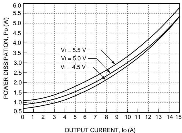
Figure 49. NH050F-L Typical Power Dissipation vs. Output Current, T_A = 25\text{ }^{\circ}\text{C}
