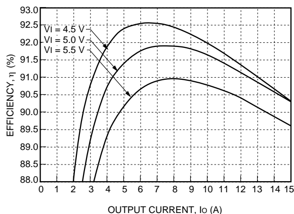
Figure 24. NH050F-L Efficiency, T_A = 25\text{ }^{\circ}\text{C}
