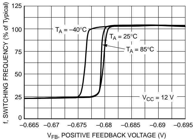
Figure 9. Switching Frequency versus Positive Feedback Voltage
