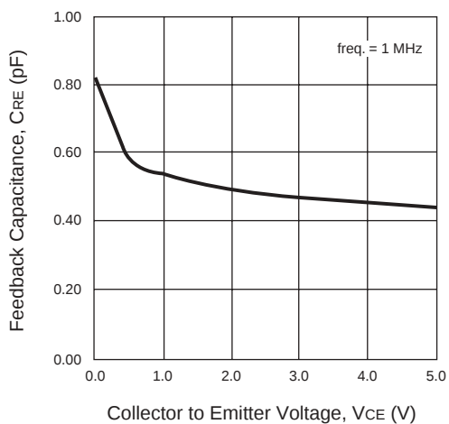
FEEDBACK CAPACITANCE vs. COLLECTOR TO EMITTER VOLTAGE
