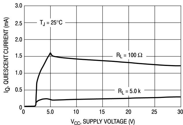
Figure 14. Quiescent Current versus Supply Voltage
