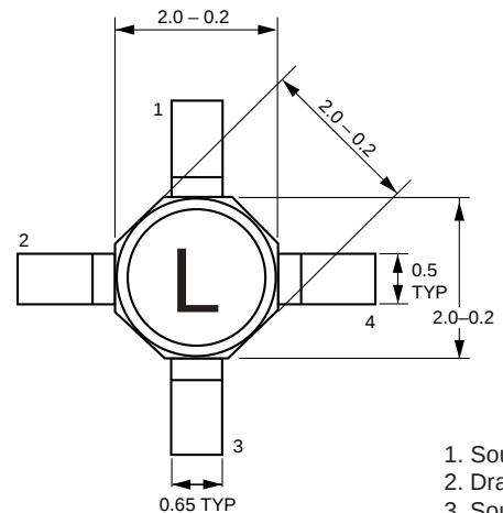
PACKAGE OUTLINE S01
