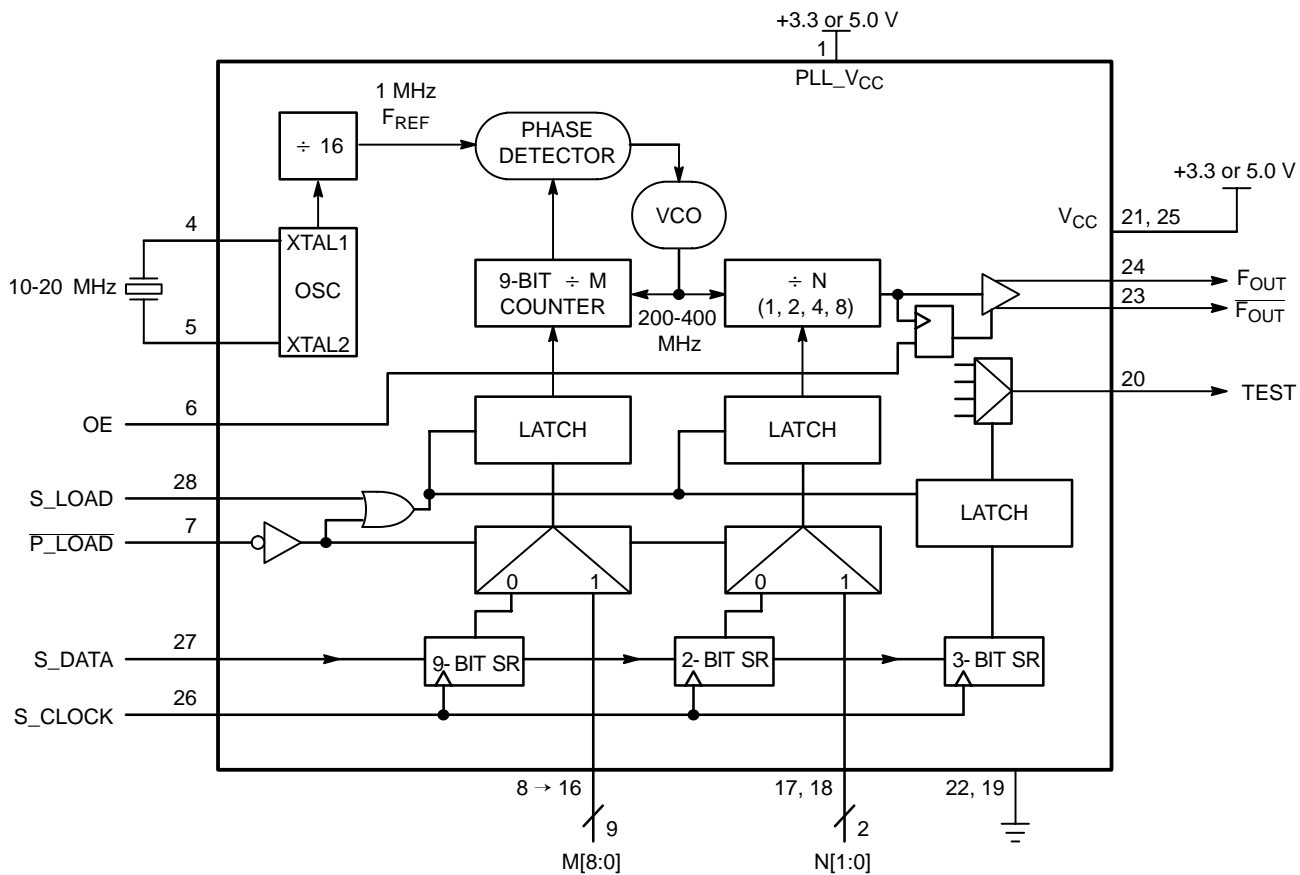
Figure 1. NBC12429 Block Diagram (28-Lead PLLC)
