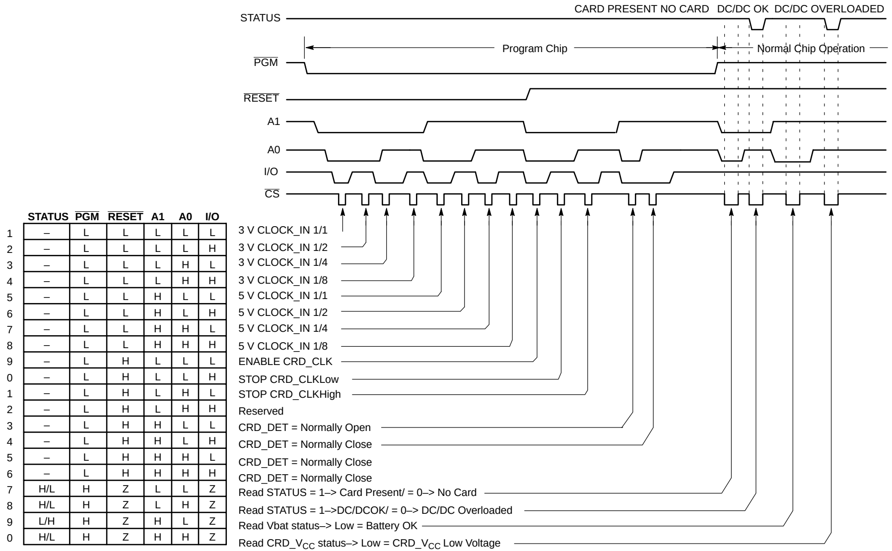
Figure 4. Programming and Normal Operation Basic Timing
