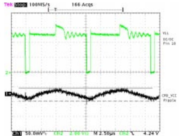
Figure 21. CRD_VCC Ripple as a Function of the Capacitor Technology
