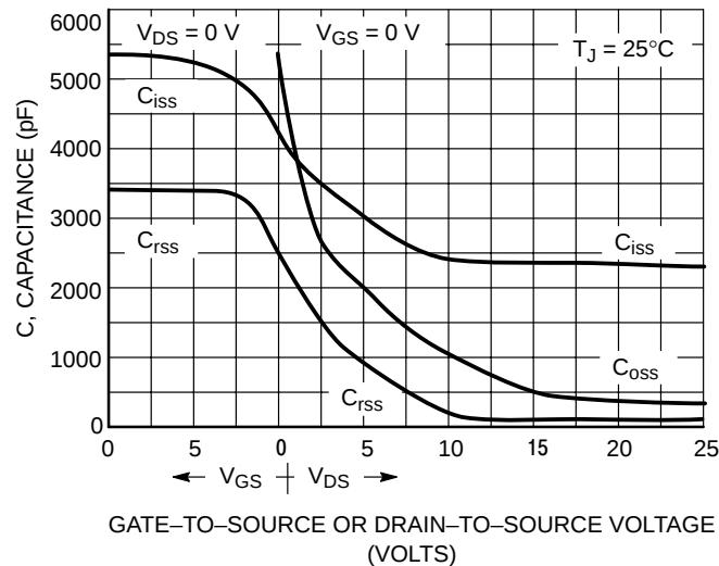
Figure 7. Capacitance Variation
