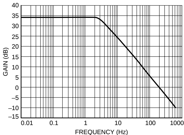
Figure 41. Forward Gain Plot
